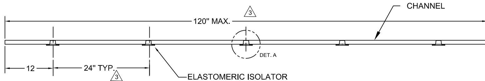
SLEEPER ELEVATION
